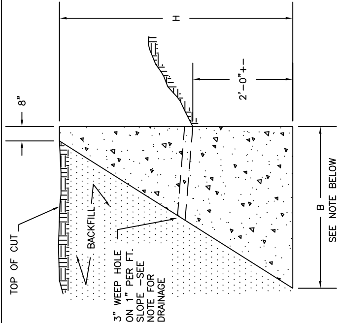
SECTION OF CONCRETE RETAINING WALL
