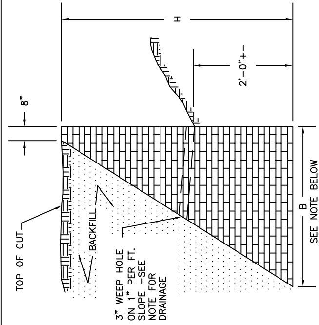
SECTION OF BRICK MASONRY RETAINING WALL
